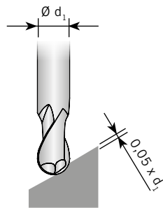
Ball nose end milling cutters
