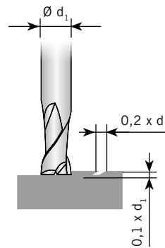
Torus end milling cutters
